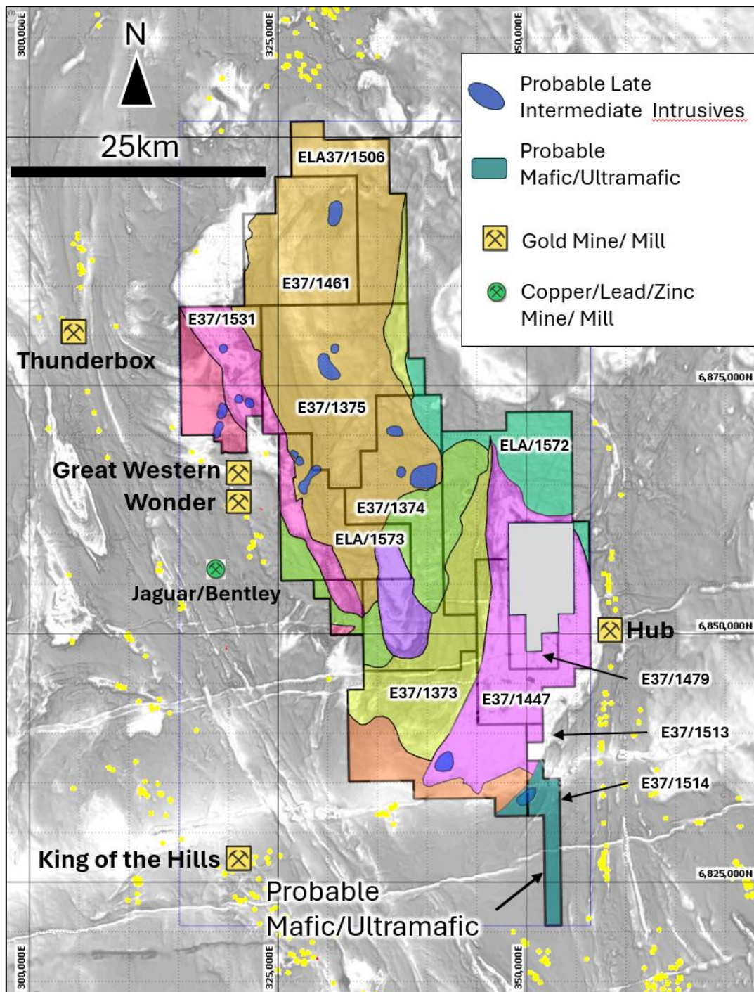
Figure 2: SensOre geophysical predictions identifying multiple intrusion types and an area of probable mafic/ultramafic rocks in the SE of the project.
